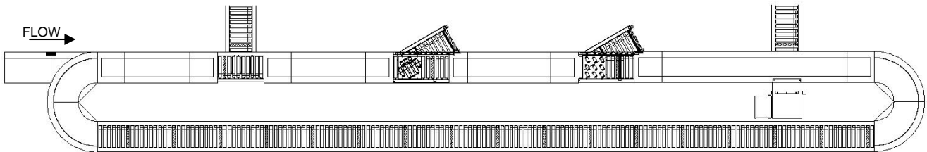
Re-circulating Sorter
